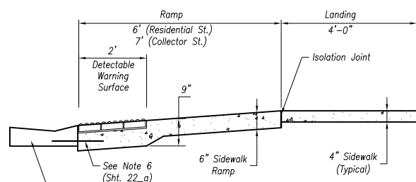
Section A-A Type B Sidewalk Ramp (Mid-Block Ramp Detail)
